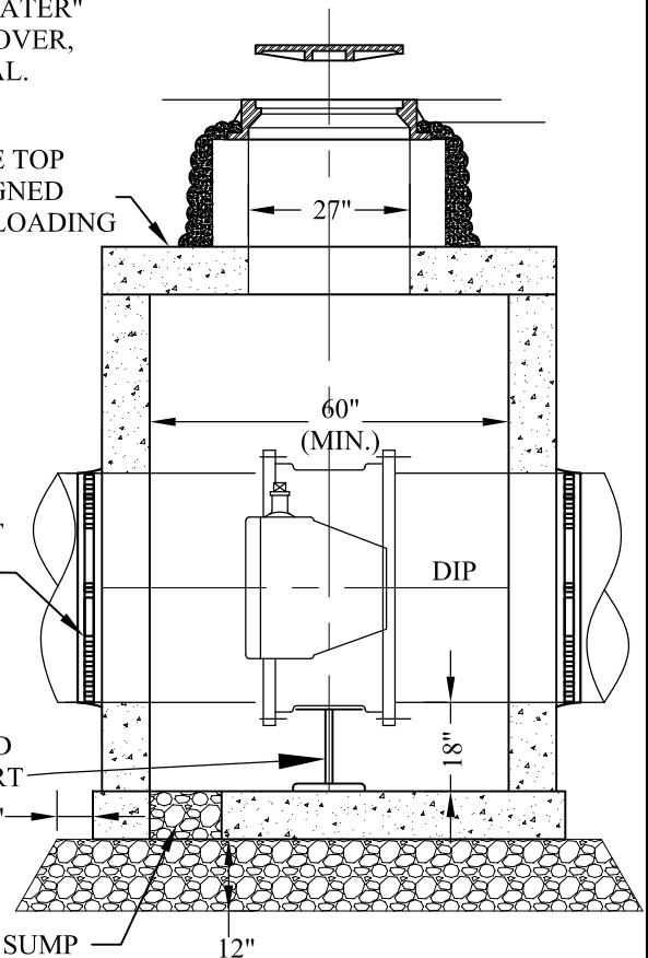
SECTION B-B
