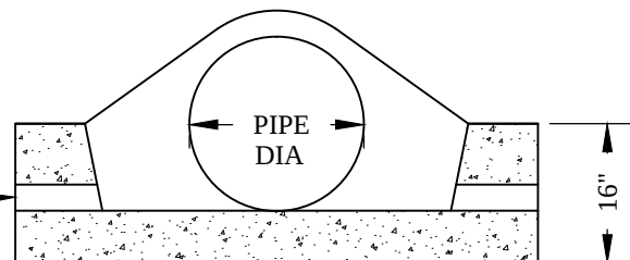
SECTION Z-Z
