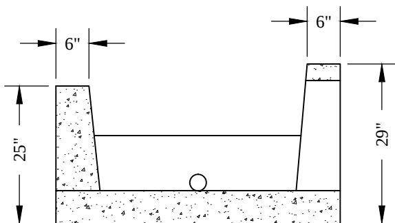
SECTION X-X
